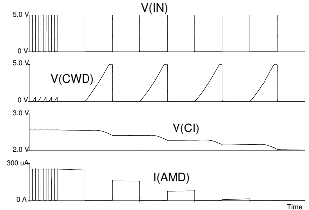
Figure 9: Watchdog, CWD open, f(\text{IN}) = 100 \text{ kHz} \rightarrow 10 \text{ kHz} (1:1), C_I = 470 \text{ nF} , R_{\text{SET}} = 10 \text{ k}\Omega
