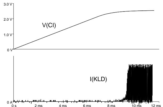
Figure 5: Turn-on behaviour, f(IN) = 100 \text{ kHz} (1:1), CI = 470 nF, RSET = 10 k \Omega
