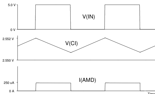
Figure 3: Steady-state APC, f(IN) = 100 \text{ kHz} (1:1), CI = 470 nF, RSET = 10 k \Omega
