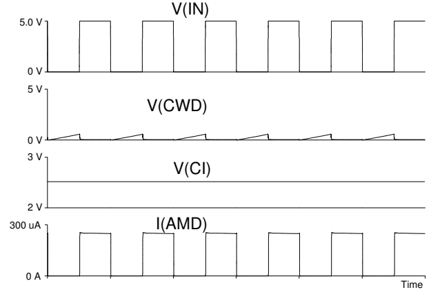
Figure 8: Watchdog, CWD open, f(\text{IN}) = 100 \text{ kHz} (1:1), C_I = 470 \text{ nF} , R_{\text{SET}} = 10 \text{ k}\Omega
