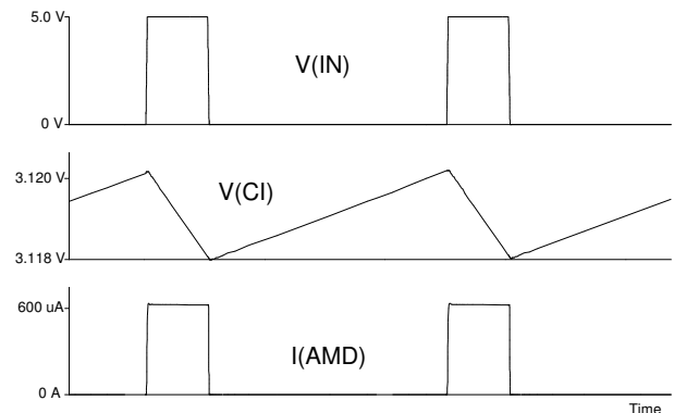
Figure 4: Steady-state APC, f(IN) = 100 \text{ kHz} (1:4), CI = 470 nF, RSET = 10 k \Omega
